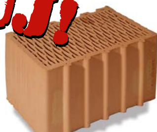
POROTHERM 38HS
